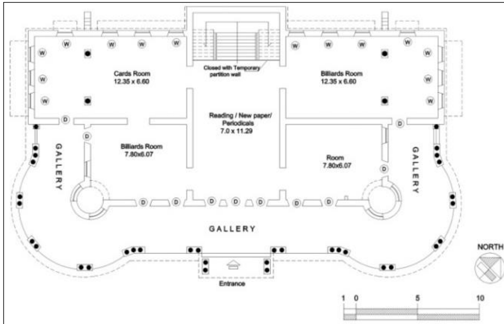
Fig. 3: Victoria Jubilee Town Hall Ground floor plan Source: Author
