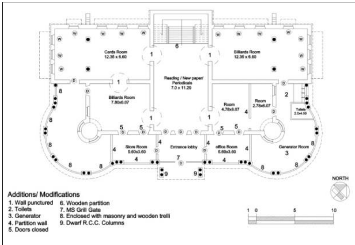
Fig. 4: Victoria Jubilee Town Hall First floor plan Source: Author
