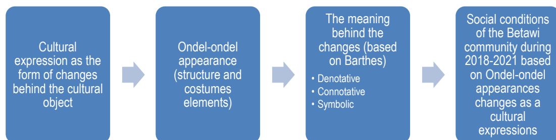
Fig. 3: Theoretical framework.
