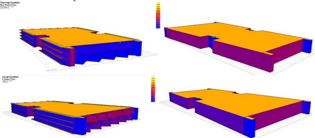
Fig. 24: Comparison of solar access between 4 sides of the building Source: Author, 2023
