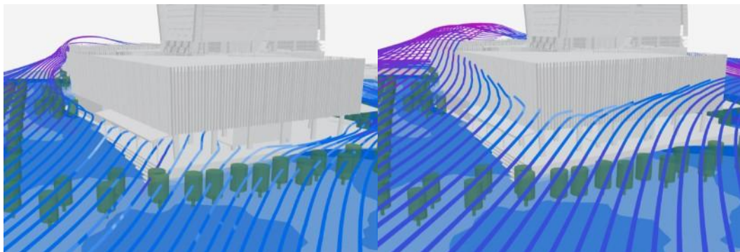
Fig. 18: Comparison of Wind movement in the northeast direction towards the walls and the building voids Source: Author, 2023
