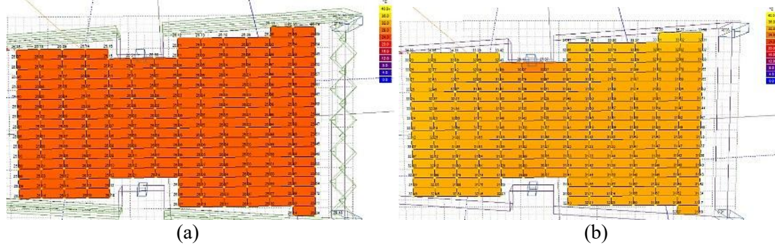
Fig. 23: Comparison Mean Radiant Temperature between (a) with shading Devices (b) without shading devices Source: Author, 2023
