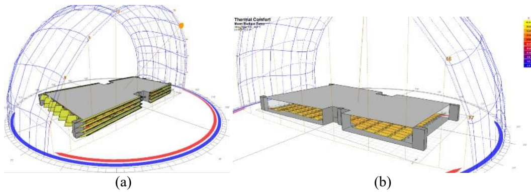
Fig. 22: 3D Modelling Comparison (a) with shading Devices (b) without shading devices Source: Author, 2023
