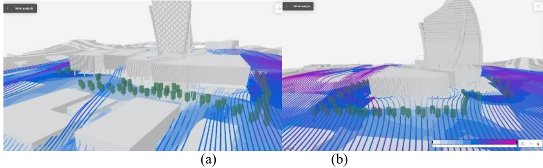
Fig. 15: (a): Wind Movement from the East of the Building, (b): Wind Movement from the North of the Building Source: Author, 2023
