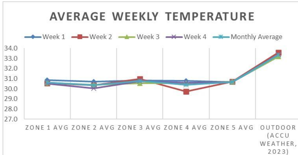
Fig. 25: Comparison of average weekly and monthly temperature between 5 Measurement Points + Outdoor
